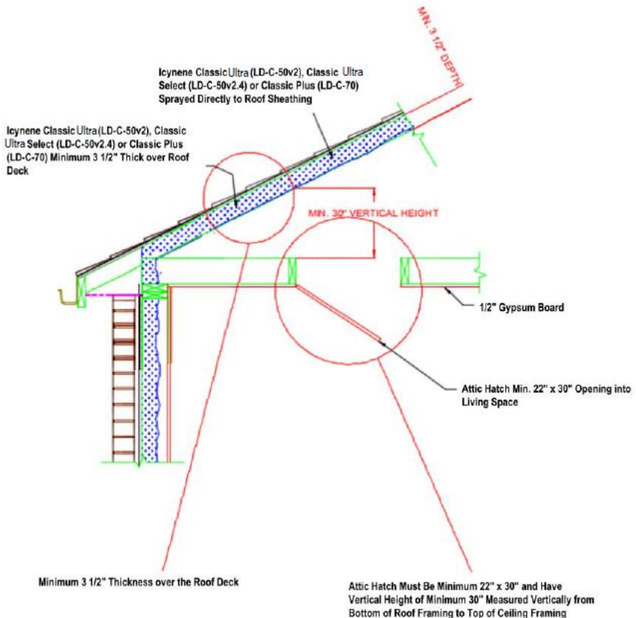
Figure 2: Icynene Classic Ultra, Classic Ultra Select & Classic Plus Used in an Unvented Attic Space
